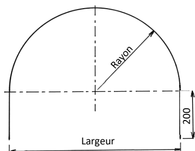
Capots 180°
